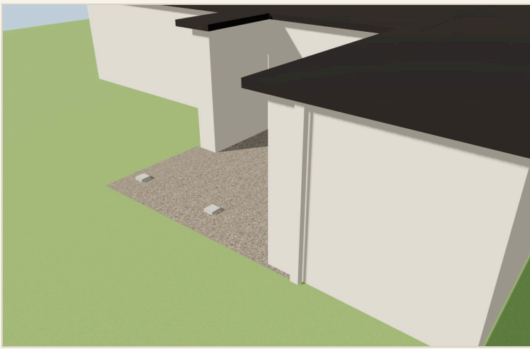
Step 1 · Footings — 3 Diamond Pier DP-50/50 driven-pin footings
